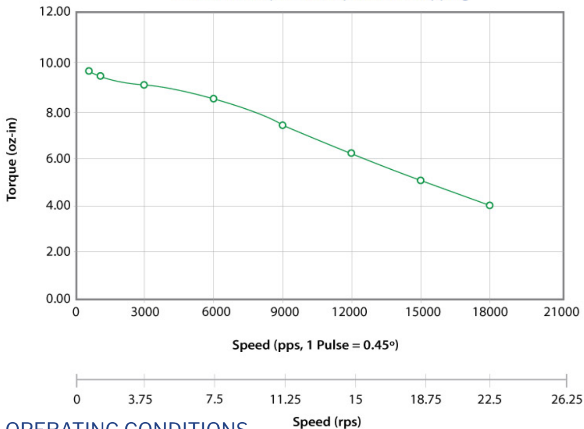
Z417-11-03 (0.9° Step Motor) 24VDC, 1.2 Amp/Phase, Bipolar, 1/2 Stepping
